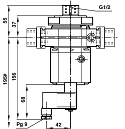
P64F Solenoid
